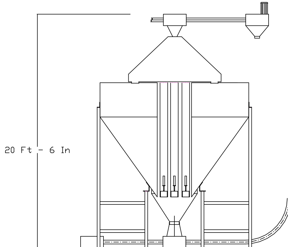
8 Hopper Storage System
